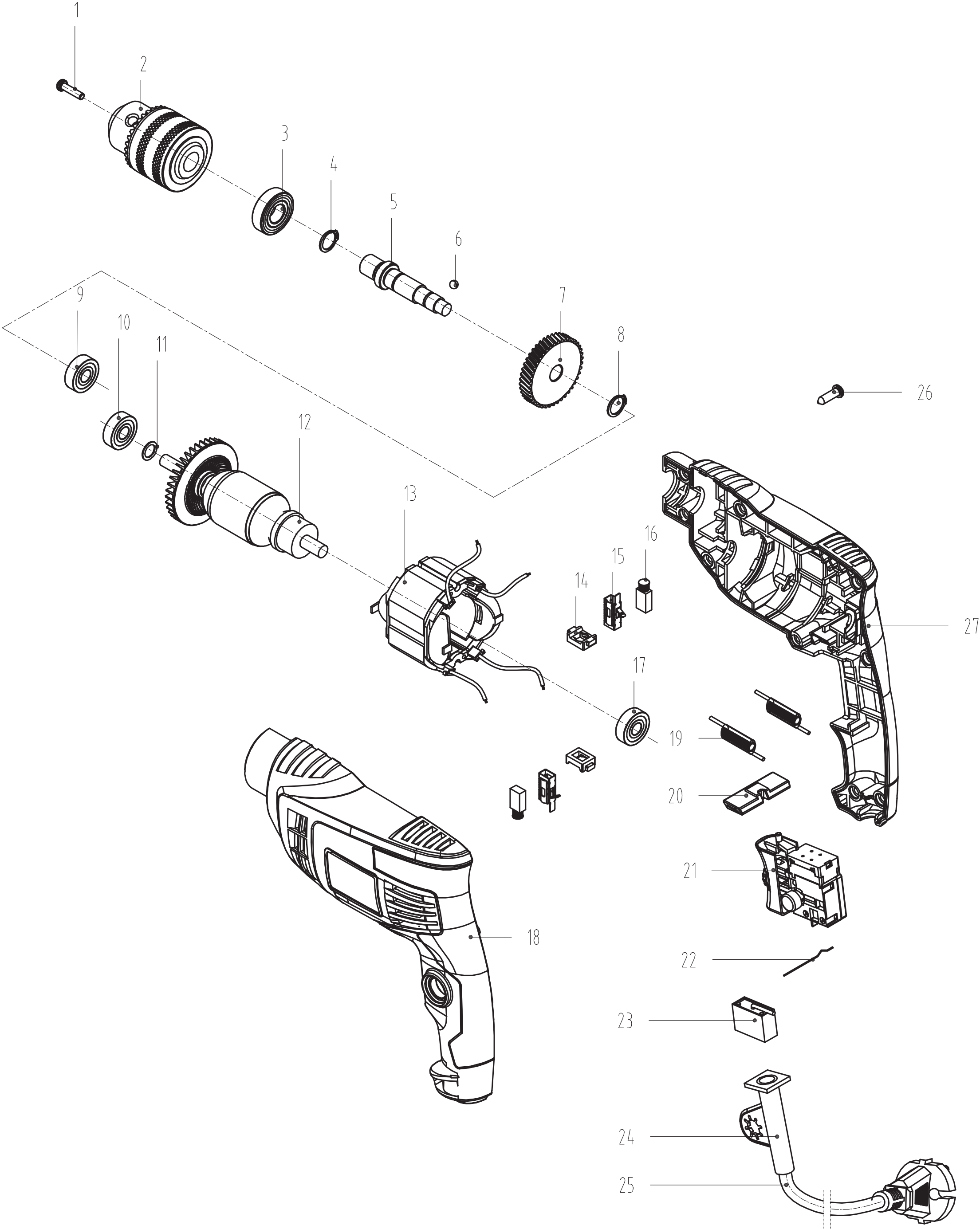
IE-ED500 (DL1006) (500W) Electric drill explosion view
